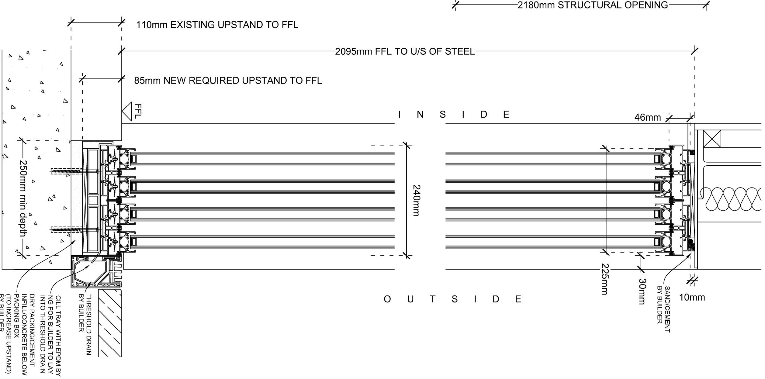
SECTION THROUGH OF SLIDE DOORS 1:20 @ A1
