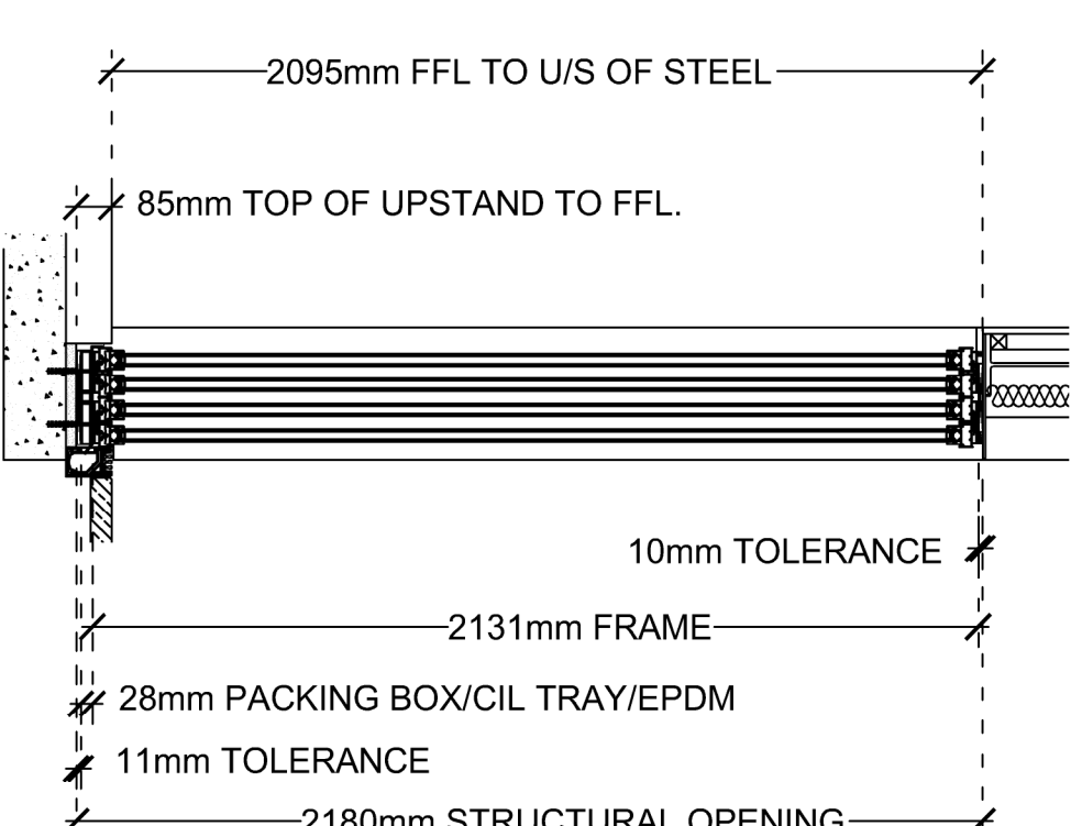
SECTION THROUGH OF SLIDE DOORS 1:20 @ A1
